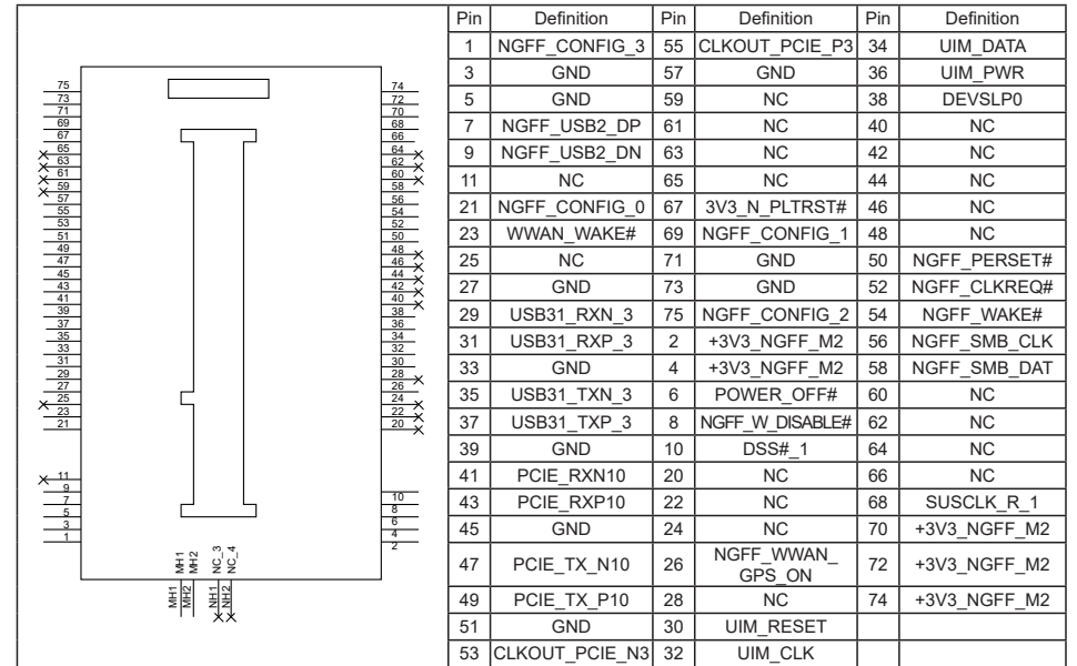
NGFF2: M.2 Key B Slot
