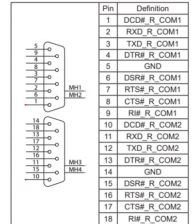
COM1: COM Port Connector
