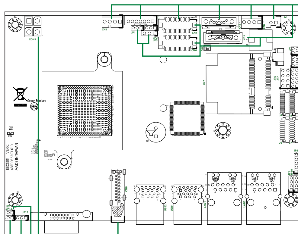
CON1: VIN Power Connector
